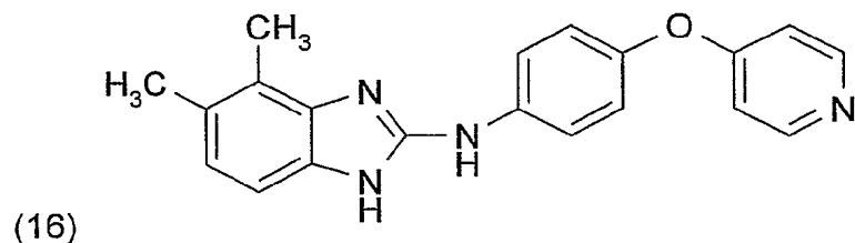
(4,5-Dimethyl-1H-benzimidazol-2-yl)-[4-(pyridin-4-yloxy)-phenyl]-amin
